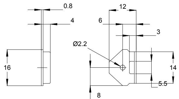
Angular Extrusion Pivot Bracket (mm)
