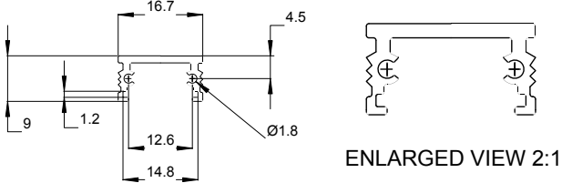
Angular Extrusion Bracket (mm)
