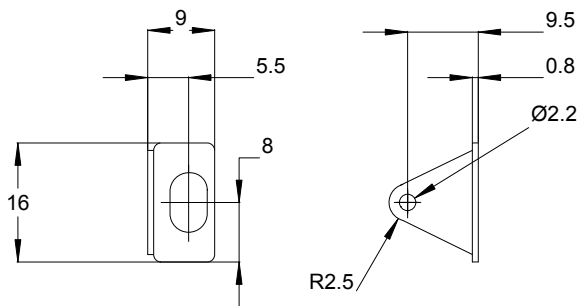
Rectangular Extrusion Bracket (mm)
