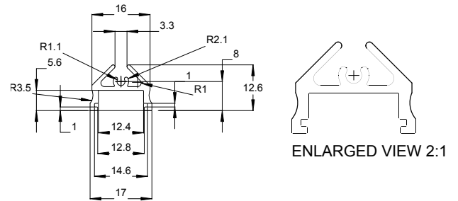
Angular Extrusion Pivot Bracket (mm)
