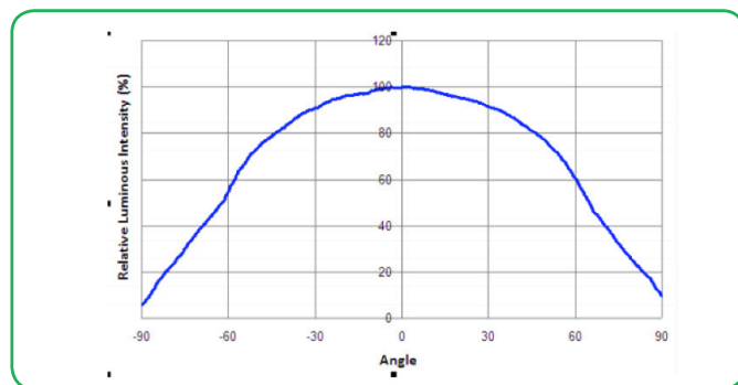
Radiation Diagram for all "XQ" products
