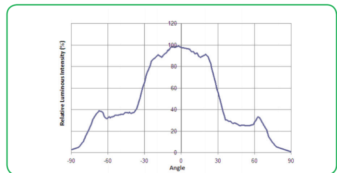
Radiation Diagram for all "XR" products
